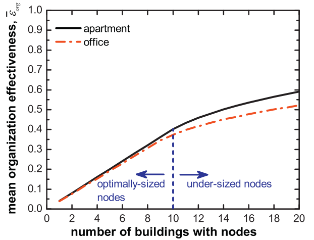
Fig. 7. Time-averaged \bar{\epsilon}_{org} as a function of the number of buildings with nodes in an organization. The analysis used an organization with 20 identical buildings, each sized with heating requirements to be 10% of the ICT power in the organization ( q_{b,req} = 0.1 P_{ICT,org} ), and the nodes underwent static loading.
