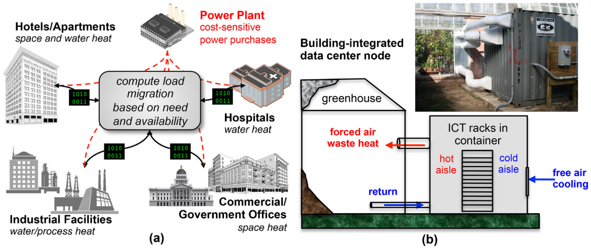
Fig. 1. (a) Schematic of EOC deployed across an organization (municipality) with EOC nodes integrated into a variety of buildings and compute jobs migrated between the nodes. (b) Schematic and photo (inset) of EOC node integrated in a greenhouse via a collaboration between the University of Notre Dame and the City of South Bend, IN. This is an air-to-space configuration where the EOC node uses free ambient air cooling and delivers the waste heat as space heat for the greenhouse.
