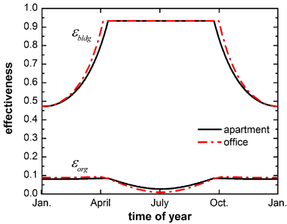
Fig. 4. Annual variations in \varepsilon_{\text{bldg}} , and \varepsilon_{\text{org}} for both an office and apartment building under static loading where P_{n,\text{ICT}} = 0.5 \cdot \max(q_{\text{b,req}}) .
