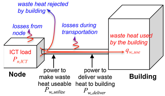
Fig. A.1. Schematic of various loss mechanisms leading to thermal inefficiencies in an EOC node/building integration.
