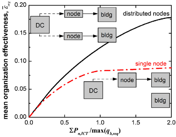
Fig. 6. Time-averaged \bar{\epsilon}_{org} as a function of the ratio of total ICT power in all nodes to the heat requirement of a single building \sum P_{n,ICT}/\max(q_{b,req}) . The case shown is for equally sized apartment buildings and nodes with static loading.
