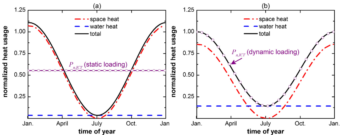
Fig. 3. Representative annual space and water heat consumption for (a) a commercial office building (inferred from [18]) and (b) an apartment building (inferred from [19]). The space heat load varies approximately sinusoidally with the maximum occurring in January and the minimum in July, whereas the water heating load is fairly constant throughout the year. The relative magnitude of the two heating types depends on the building. Also shown are the two cases of (a) static (at 50% of the peak heating requirement) and (b) dynamic ICT loading in the EOC node.
