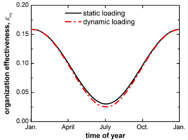
Fig. 5. Annual variations in \varepsilon_{\text{org}} for apartment building under static and dynamic loading conditions assuming a static loading condition of P_{n,\text{ICT}} = \max(q_{\text{b,req}}) .
